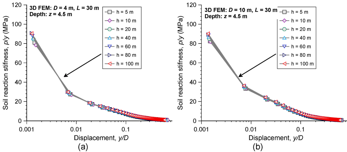
Fig. 11. Influence of loading eccentricity on pile-soil interaction: (a) p - y curves of 4 m diameter monopiles at depth z = 4.5 m; (b) p - y curves of 10 m diameter monopiles at depth z = 4.5 m.
