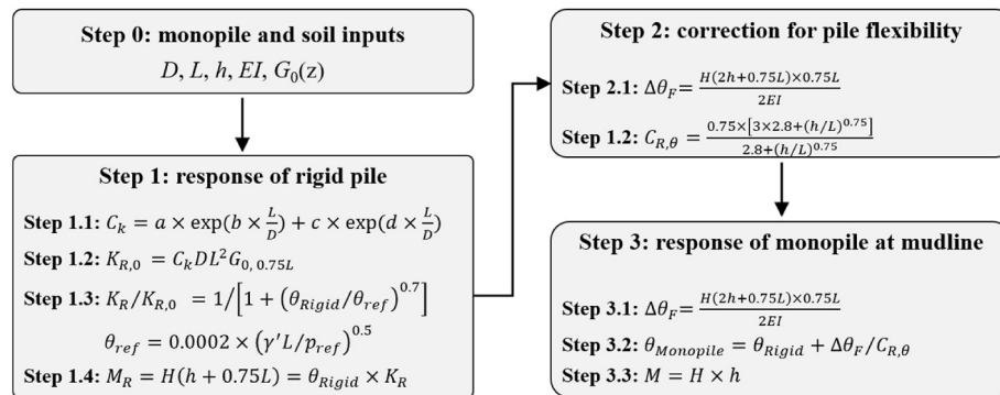
Fig. 21. Flow chart indicating the steps for calculating the moment-rotation response of monopiles.
