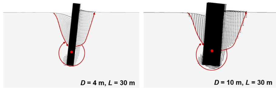
Fig. 10. Failure mechanism of the rigid monopiles in sand (Wang et al., 2022b).
